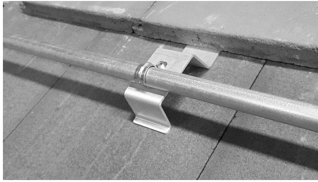
Tile Accessory Mount used in a conduit application.
