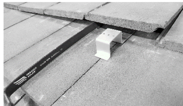
Junction Box mounted on a Tile Accessory Mount using the Pegasus Junction Box Bracket Attachment (RLUJB00AM00B-12).
