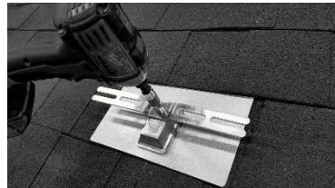
1. Comp: Install conduit mount per instructions. Thread lag through junction box bracket with EPDM washer on mount and drive lag.
