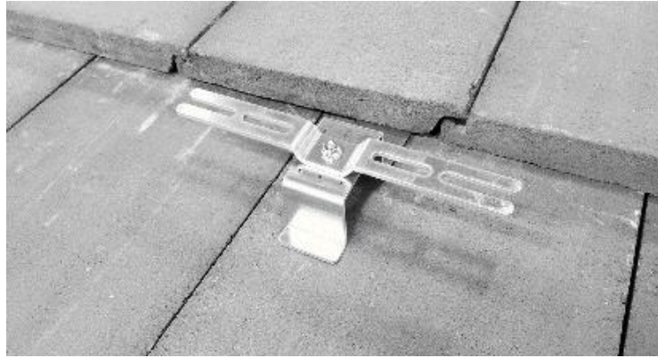
Junction Box mounted on a Tile Accessory Mount using the Pegasus Junction Box Bracket Attachment.
