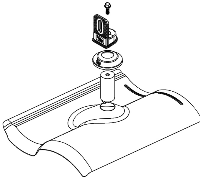
Diagram LF2: Pegasus Solar™ L-Foot on Pegasus Tile Replace Mount
